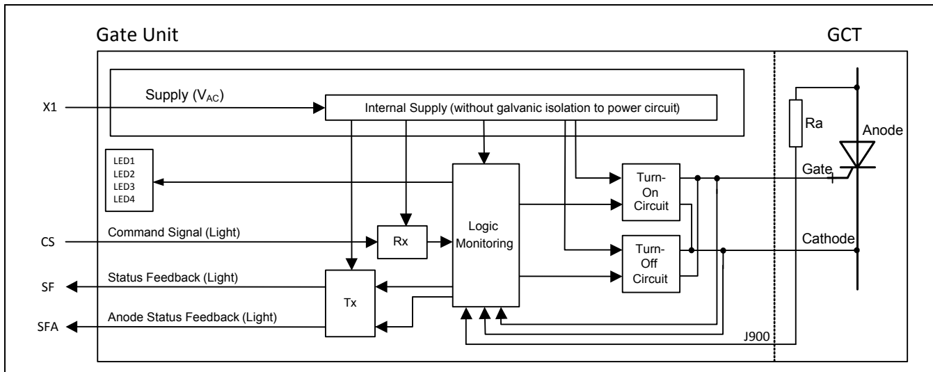
Fig. 13 Block diagram
